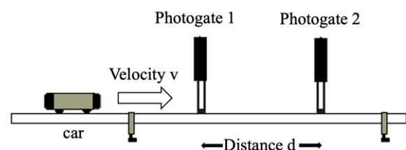
Figure 4.2 An Experiment Setup for a Measurement of An Instantaneous Velocity Using Photogate Timers.
