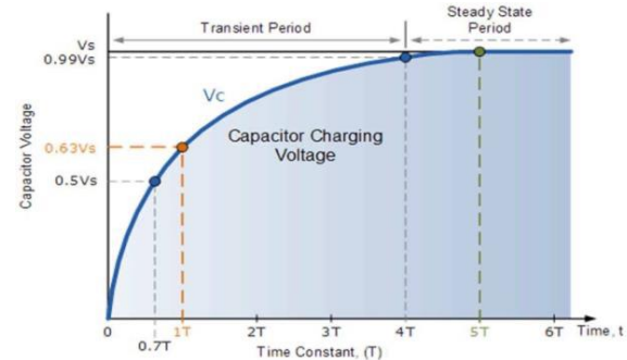
Figure 1.2 Showing a Curve of Charging Voltage as a Function of Charging Time of RC Circuit
