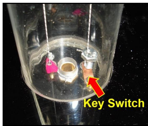
Figure 2.2 Showing a Micro-Key Switch in the Chamber for Triggering the Electronic Circuit of Time
