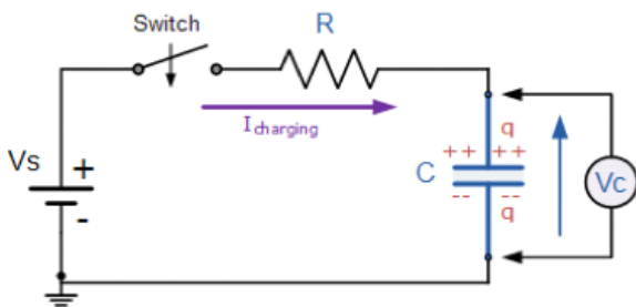
Figure 1.1 Showing A Circuit Diagram for RC-Charging
